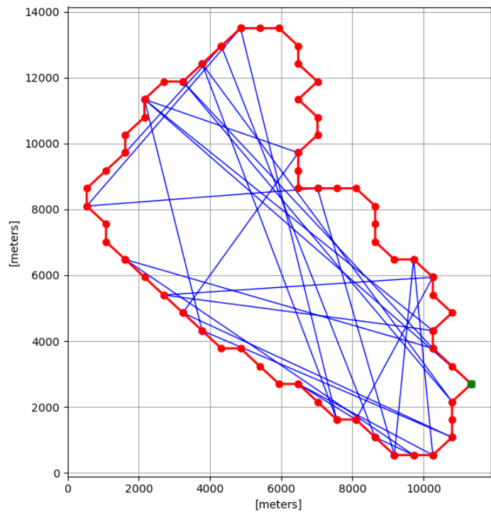
Fig. 4.20 Random solution
