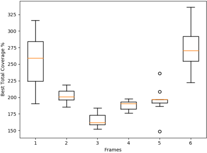
Fig. 5.7 Boxplot of multiples simulations
