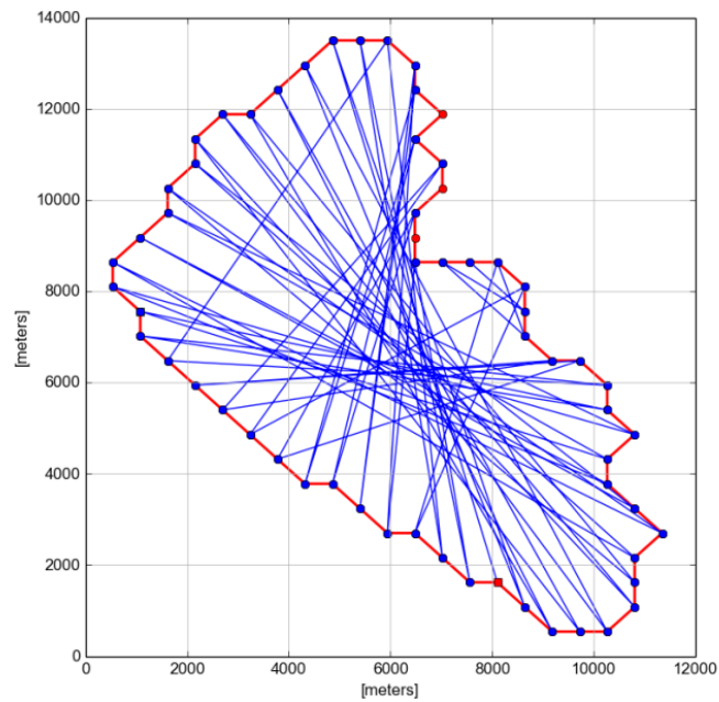
Fig. 4.15 Greedy algorithm
