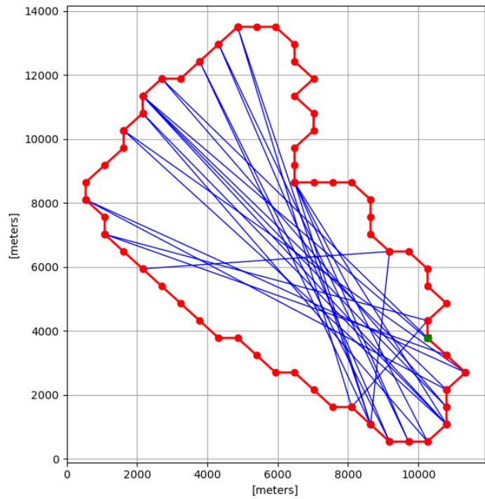
Fig. 4.21 Eulerian Solution
