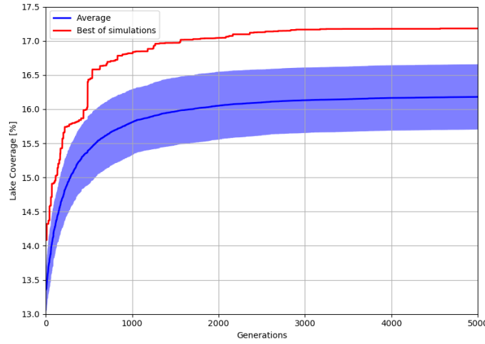
Fig. 4.18 Evolution of the best individual ( Cx = 0.8 , mut = 0.2 )
