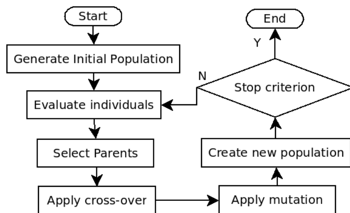
Fig. 3.5 Illustration of GA steps
