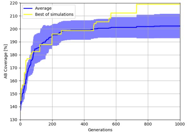
Fig. 5.9 Evolution of solutions - frame 2
