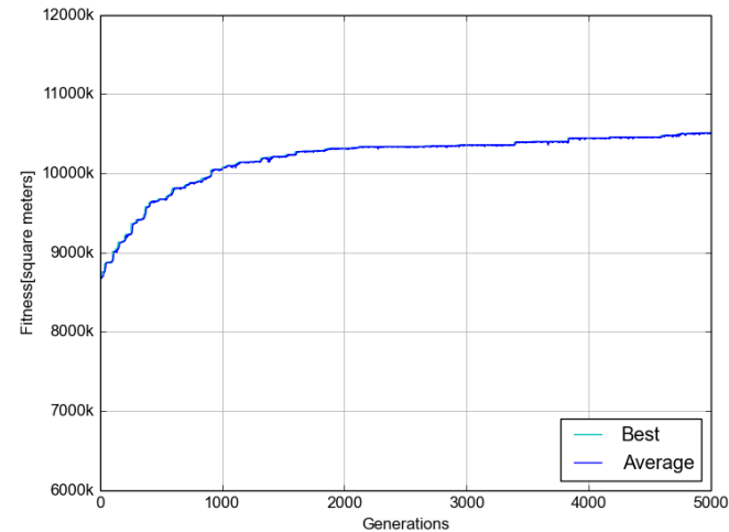
Fig. 4.12 GA with restriction PF (constrained) - Evolution
