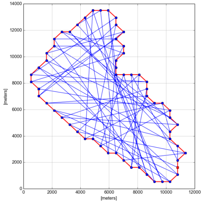
Fig. 4.14 Randomized algorithm
