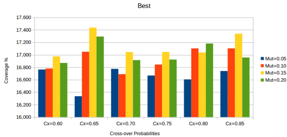
Fig. 4.17 Best solutions of all simulations
