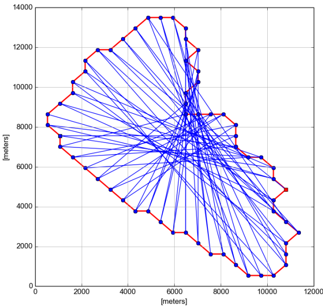
Fig. 4.7 GA with no restriction (unconstrained) - Best individual
