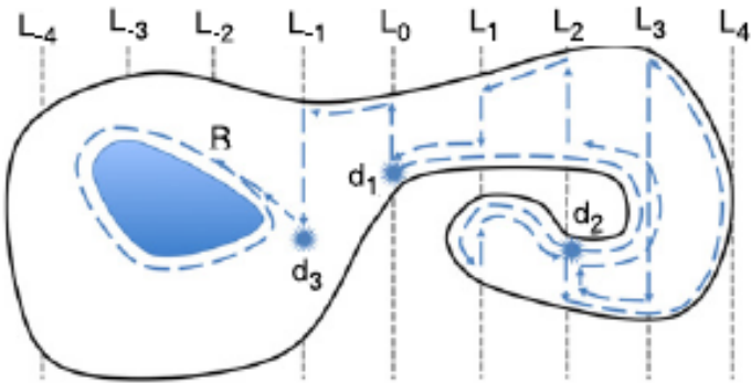
Fig. 2.11 Semi-approximate map
