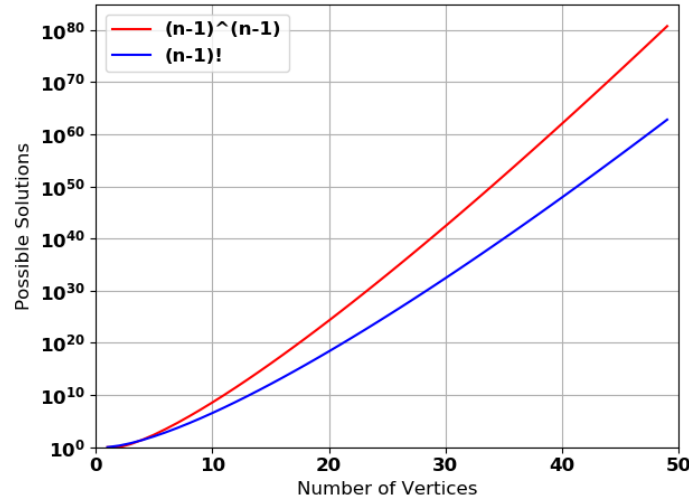
Fig. 3.4 Complexity of Eulerian Circuit ((n-1)^{(n-1)}) vs Hamiltonian Circuit (n-1)!
