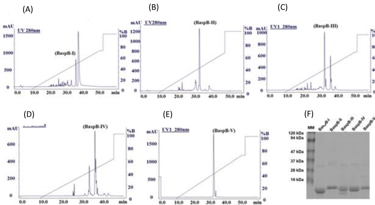
Fig. 4. Isolation of five basic PLA 2 isoforms: RPC of the basic fractions (CM7-CM11) from the IEC permitted the isolation of five basic PLA 2 s, called BaspB-I, BaspB-II, BaspB-III, BaspB-IV and BaspB-V (A–E). The electrophoretic profile showed a relative molecular mass of 14 kDa for the purified proteins, compatible with this group of proteins (F).
