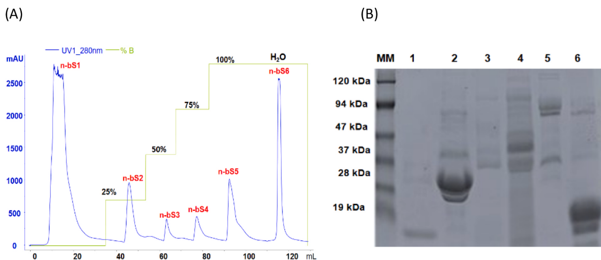
Fig. 2. Fractionation of CM2 in HIC: Six fractions, named n-bS1 to n-bS6, were eluted (A). In the electrophoretic profile (B), the relative molecular mass of the proteins present in the eluted fractions can be observed. Fraction n-bS6, which eluted with water, presented proteins with molecular masses compatible with those of PLA 2 s. This fraction was selected for the next step.
