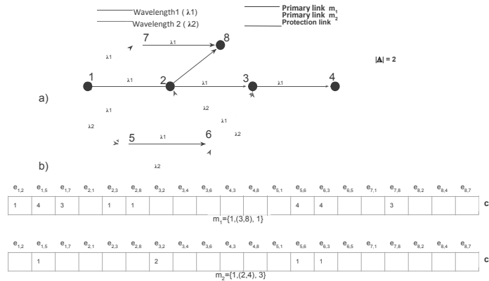
Fig. 1. Representation of a solution C = \{c_1, c_2\} . a) Solution on a light-graph, b) Chromosome. Note that nodes 2 and 3 are splitter nodes while node 3 is, in addition, a wavelength converter. The light-links used by protection light-paths have a number of \lambda > |A| to differentiate them from the primary light-links.
